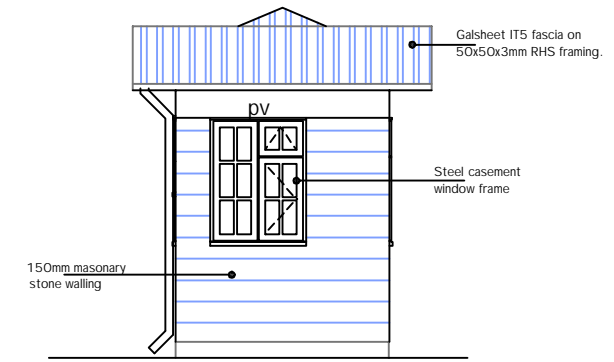
ELEVATION 03
