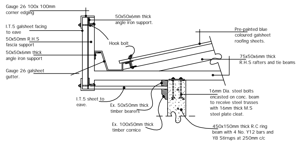
EAVE DETAIL
